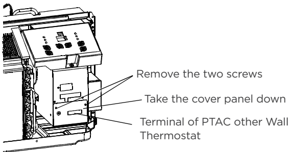
Terminal of PTAC Wall Thermostat (MODE A)
