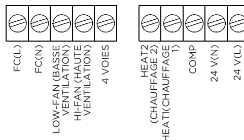
Borne du thermostat mural PTAC (MODE A)
