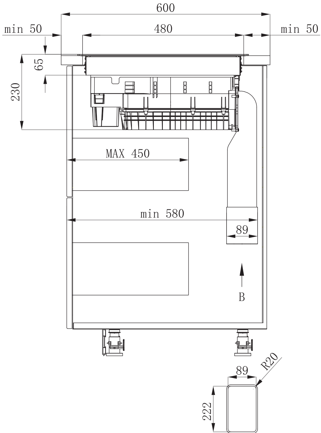
B VIEW: Adapter dimension
