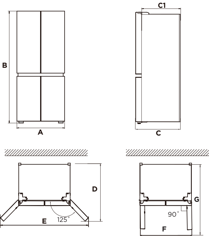
Space requirement diagram (when the door is open and when the door is closed)
