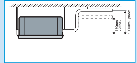
Built-in Drain Pump
