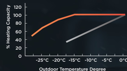
M-Powevi Multi-split System Heating Capacity At Low Temperature
