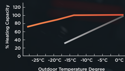
M-Powevi Single-split System Heating Capacity At Low Temperature
